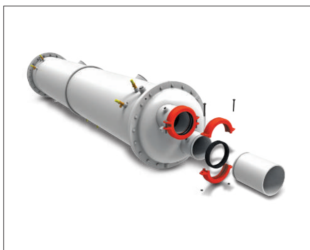
Victaulic connections
